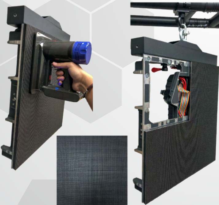
FRONT SERVICEABLE
